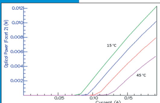
Laser I curves showing T-dependence
